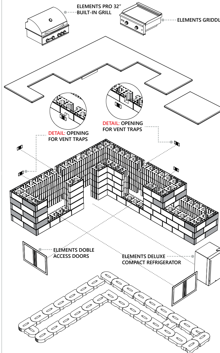
EXPLODED VIEW
