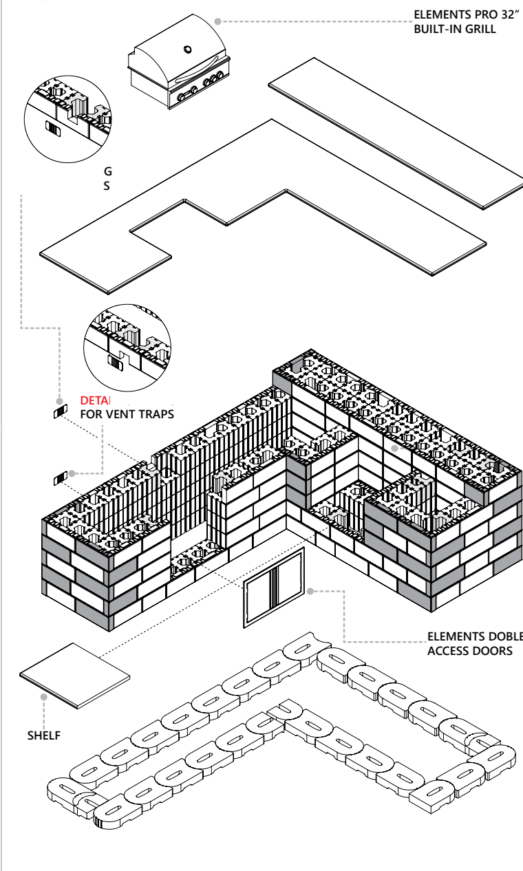
EXPLODED VIEW
