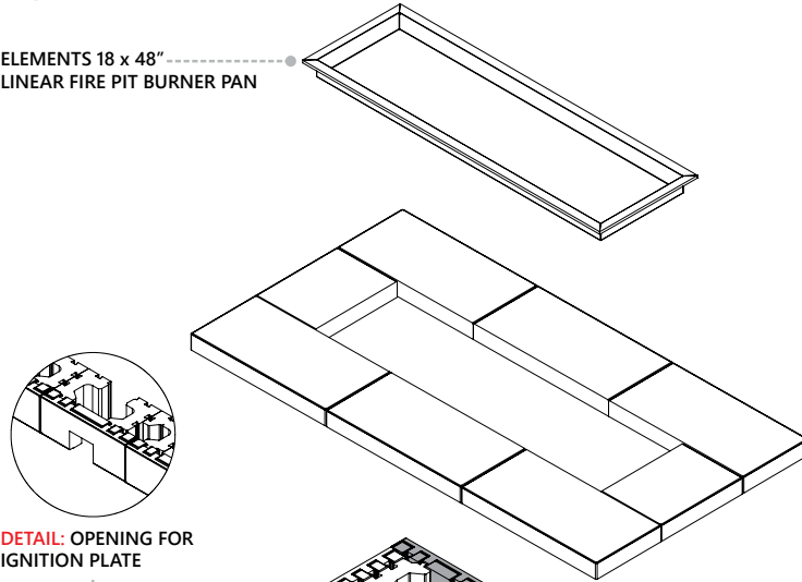
EXPLODED VIEW
